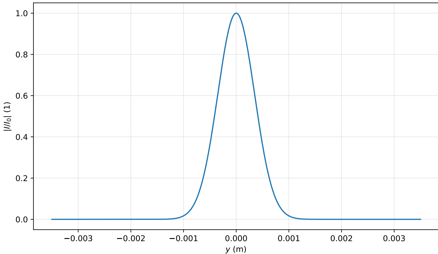
Intensity profile I(x=0, y, z=0.000)/I_0 , \text{Pin}=0.7\text{Pcr} , artificial time
